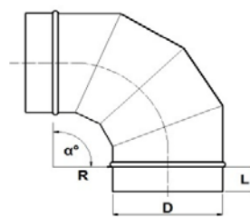
d80-d900 / L=50mm
